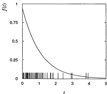
Fig. 6.2 A sample of 50 Monte Carlo generated observations of an exponential random variable t with mean \tau = 1.0 . The curve is the result of a maximum likelihood fit, giving \hat{\tau} = 1.062 .
