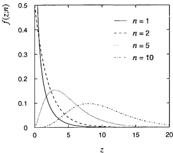
Fig. 2.7 The \chi^2 probability density for various values of the parameter n .
